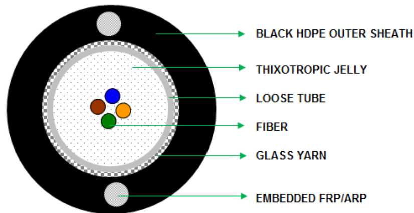
Figure 1: Typical Structure Drawing for 4 Fibre Cable
